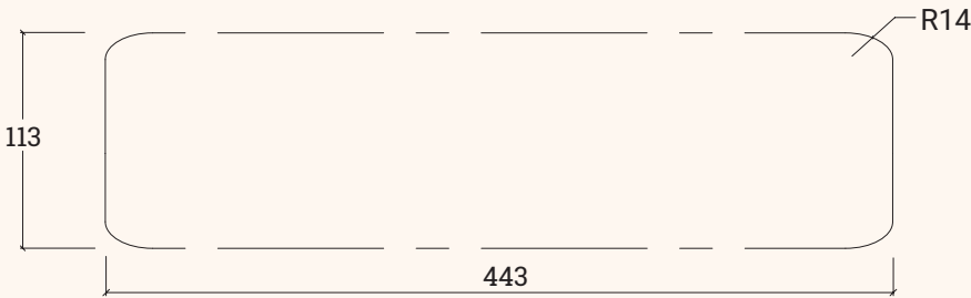
Drilling pattern
