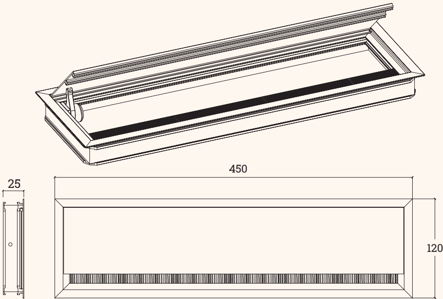
Technical Drawings
