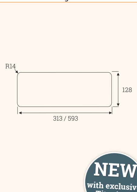
Drilling Pattern
