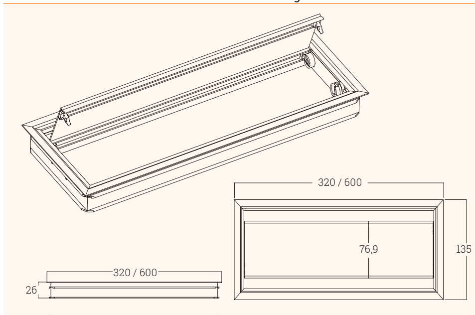
Technical Drawing
